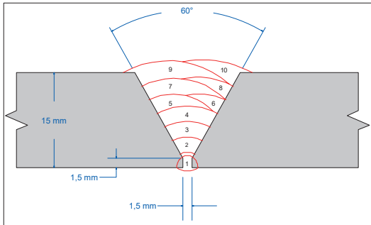
Fully SMAW procedure welding sequence
