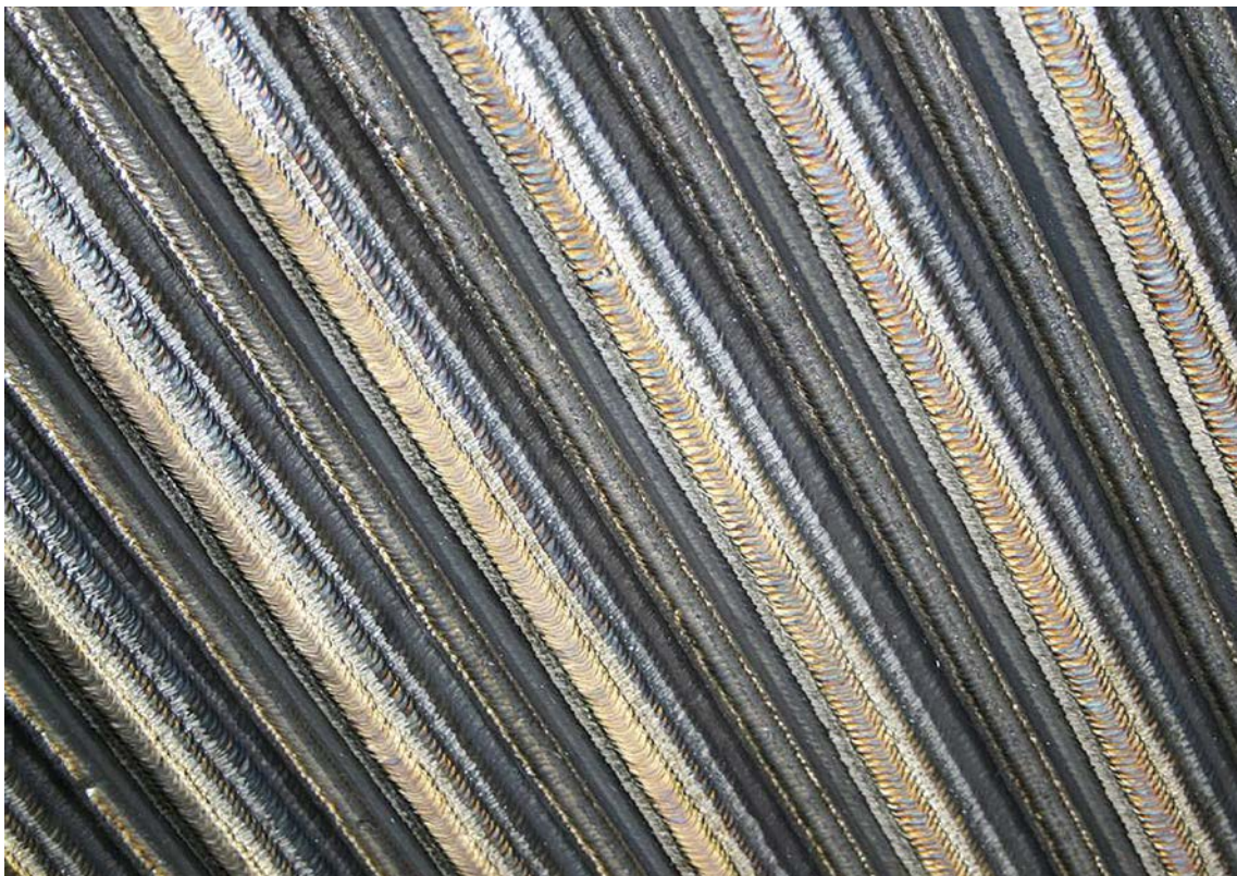
Membrane wall clad with Alloy 625
